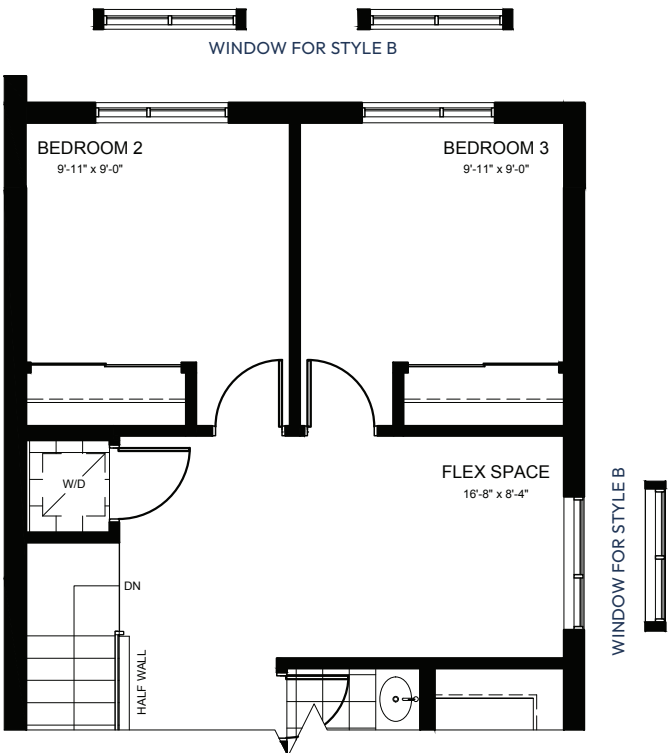
PARTIAL ALT. THIRD FLOOR STYLE A & B
