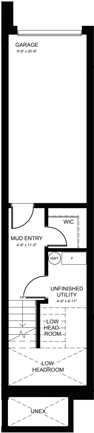
LOWER FLOOR STYLE A & B
