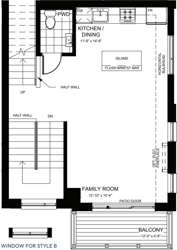
SECOND FLOOR STYLE A & B
