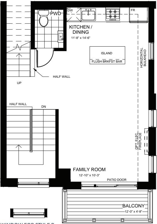
SECOND FLOOR STYLE A & B
