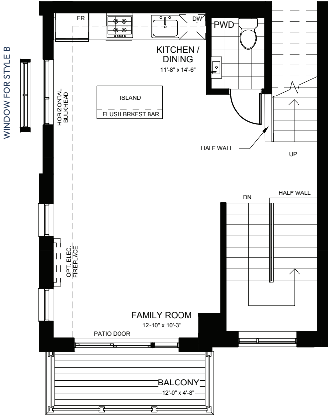
SECOND FLOOR STYLE A & B
