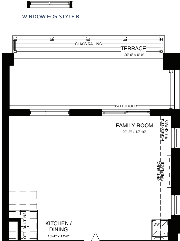
PARTIAL ALT. FIRST FLOOR STYLE A & B
