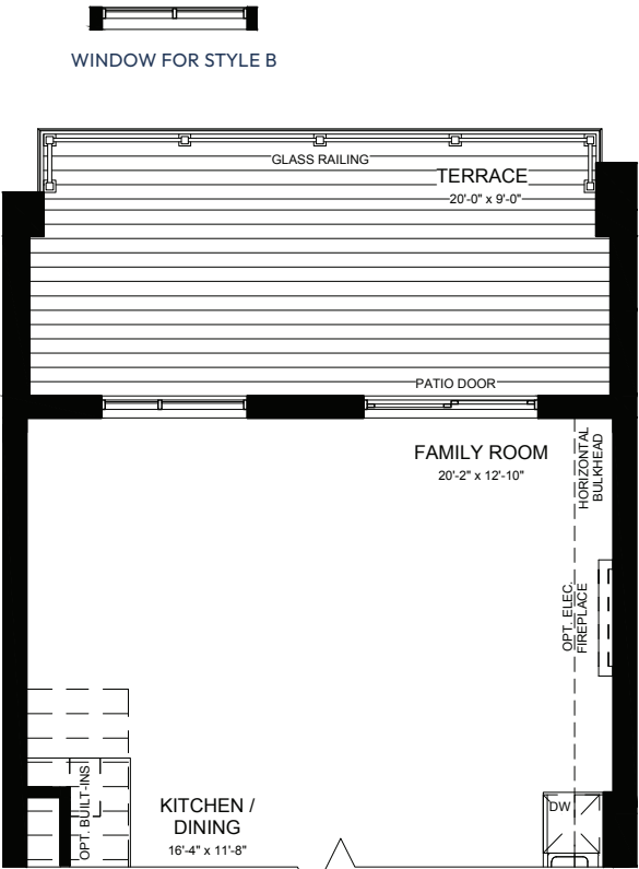
PARTIAL ALT. FIRST FLOOR STYLE A & B
