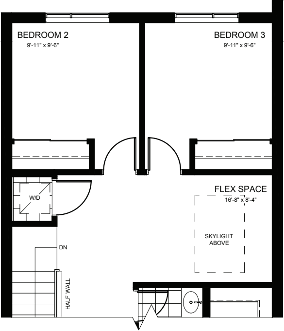
PARTIAL ALT. THIRD FLOOR STYLE A & B
