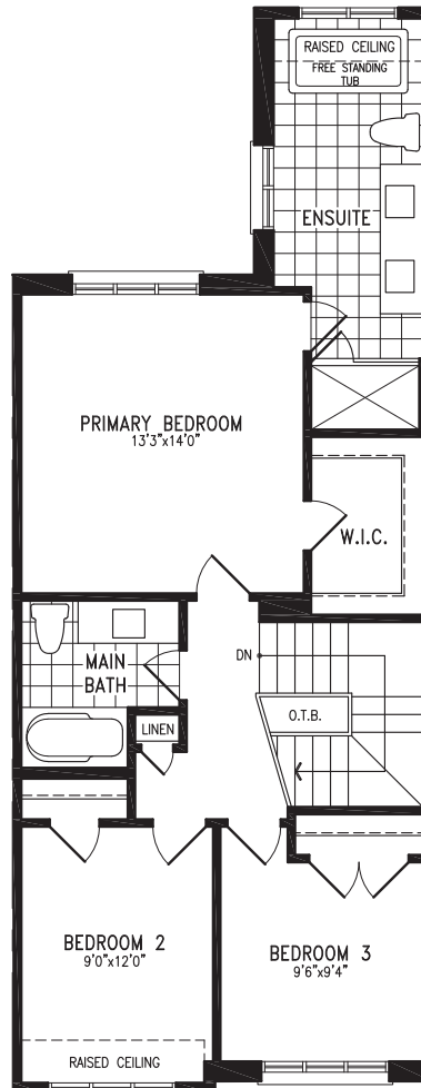
Elevation A SECOND FLOOR
