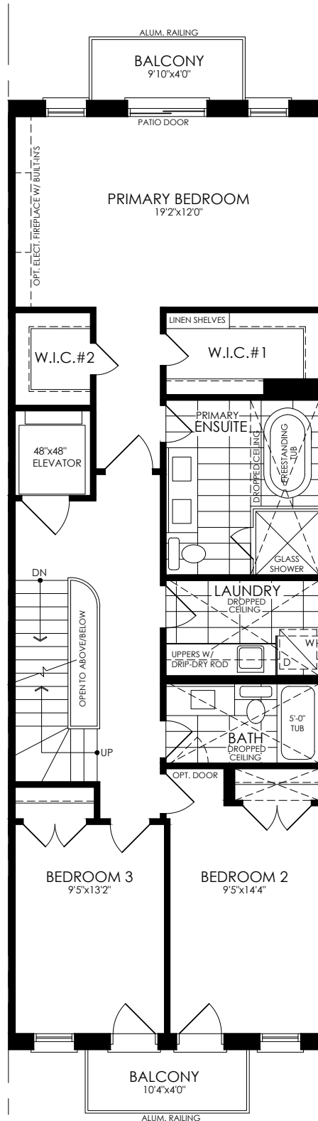
OPTIONAL THIRD FLOOR • ELEV. A
