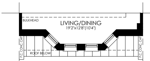
PARTIAL SECOND FLOOR • ELEV. B
