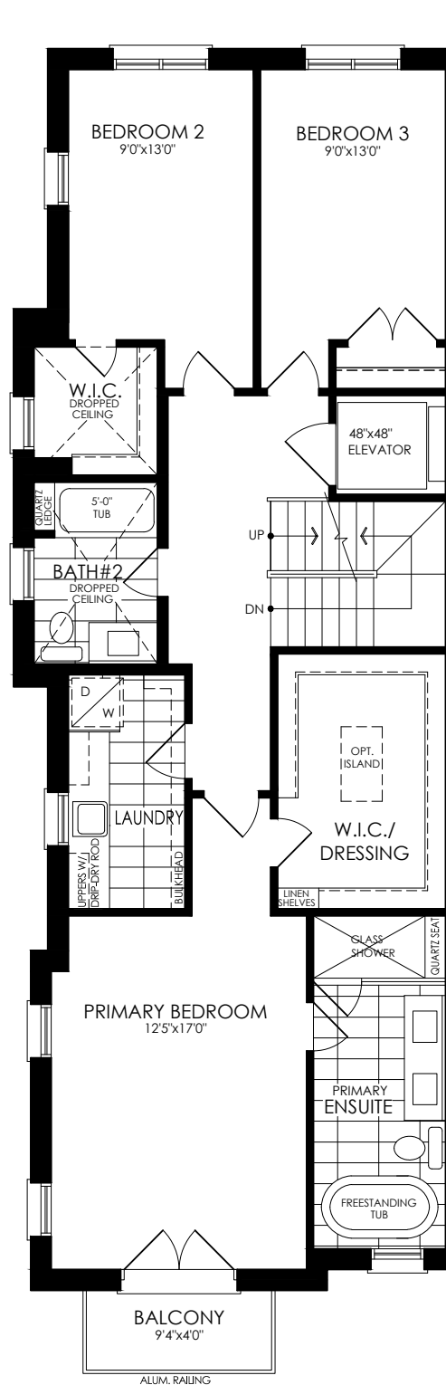
THIRD FLOOR • ELEV. A
