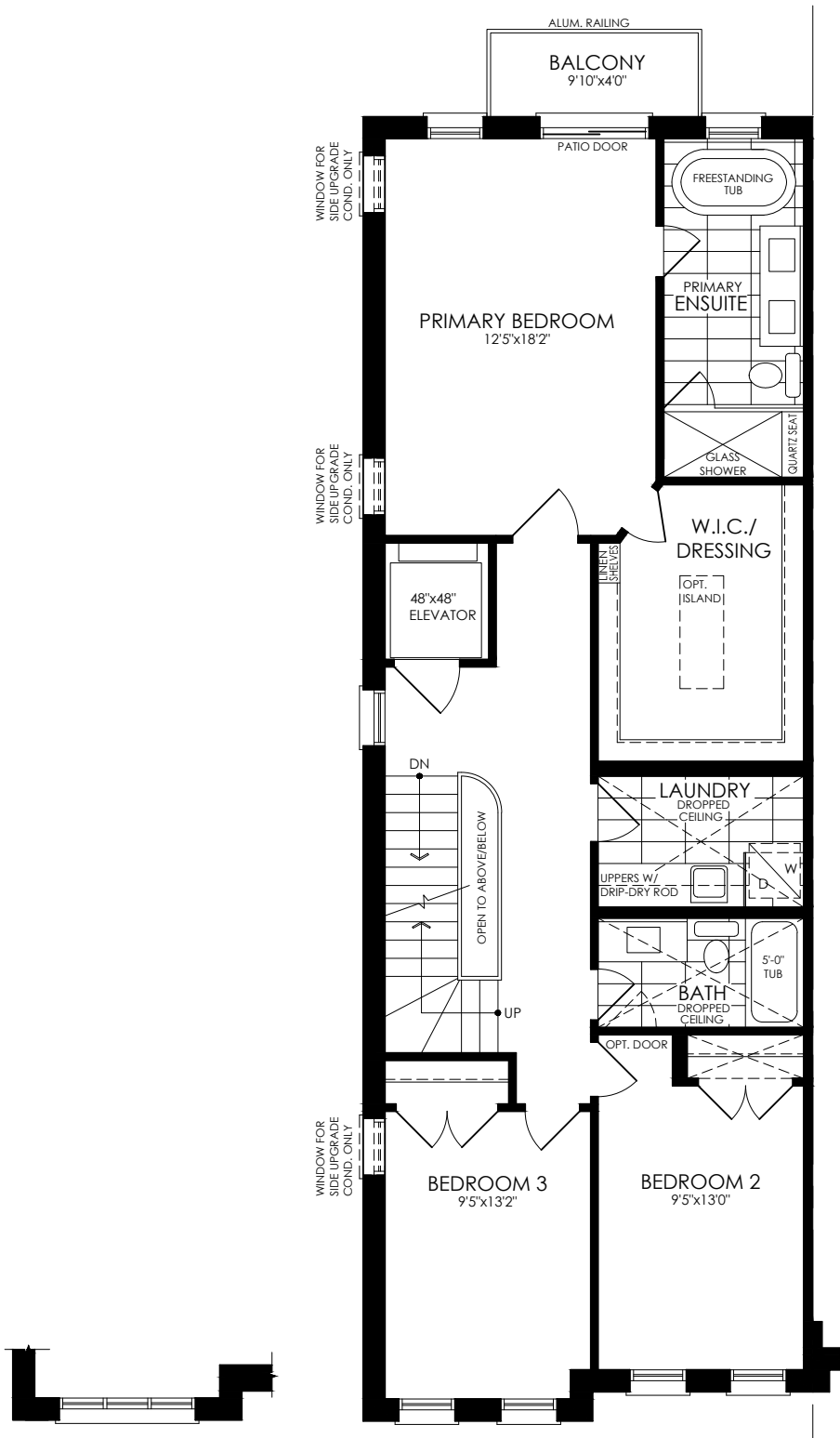
PARTIAL THIRD FLOOR • ELEV. B
