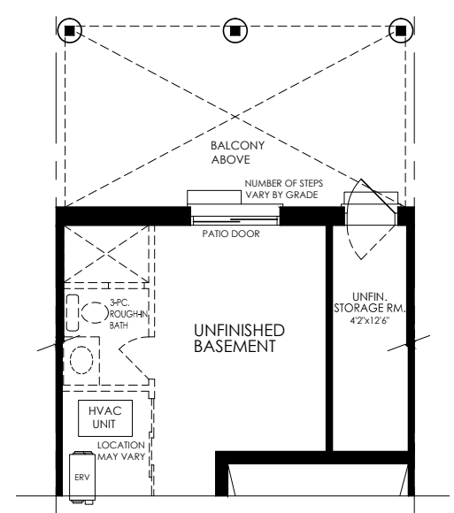
PARTIAL BASEMENT W/ WALK-OUT BASEMENT COND. • ELEV. A
