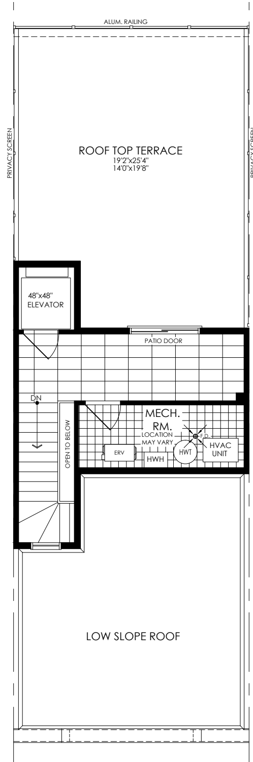
ROOFTOP/TERRACE • ELEV. A
