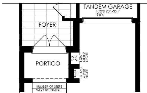
PARTIAL GROUND FLOOR • ELEV. B
