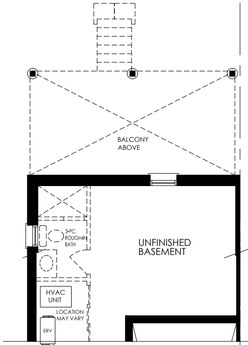
PARTIAL BASEMENT W/ WALK-OUT DECK COND. • ELEV. B
