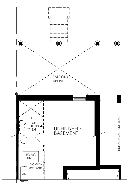
PARTIAL BASEMENT W/ WALK-OUT DECK COND. • ELEV. A
