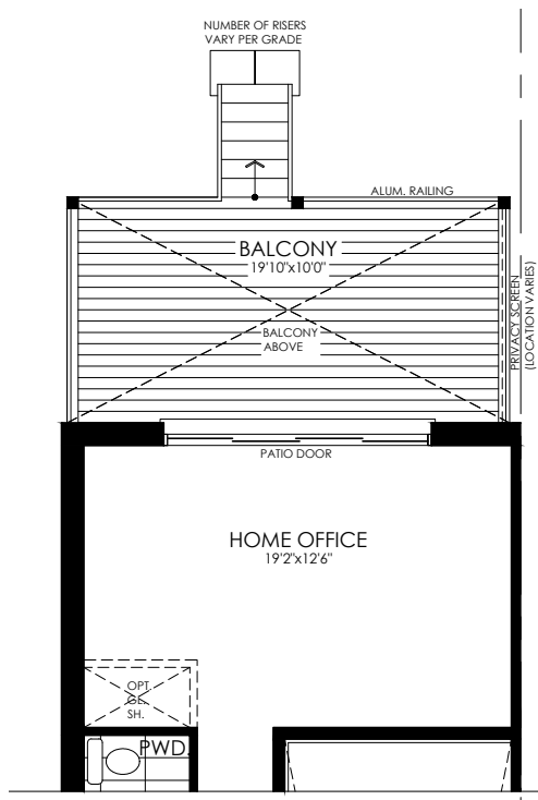
PARTIAL GROUND FLOOR W/ WALK-OUT DECK COND. • ELEV. B
