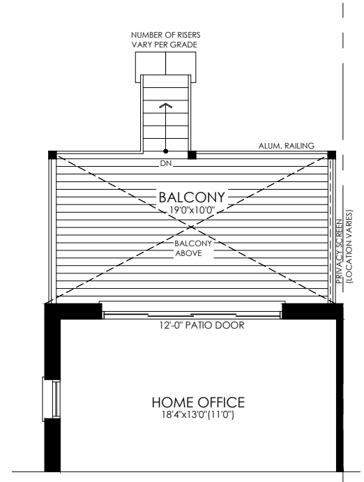
PARTIAL GROUND FLOOR W/ WALK-OUT DECK COND. • ELEV. A
