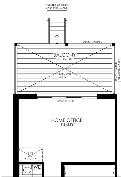
PARTIAL GROUND FLOOR W/ WALK-OUT DECK COND. • ELEV. C
