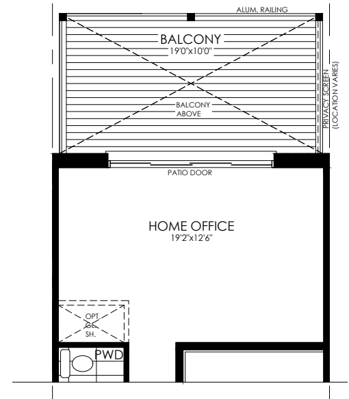
PARTIAL GROUND FLOOR W/ WALK-OUT BASEMENT COND. • ELEV. A
