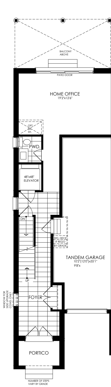
PARTIAL GROUND FLOOR W/ WALK-OUT BASEMENT COND. • ELEV. A
