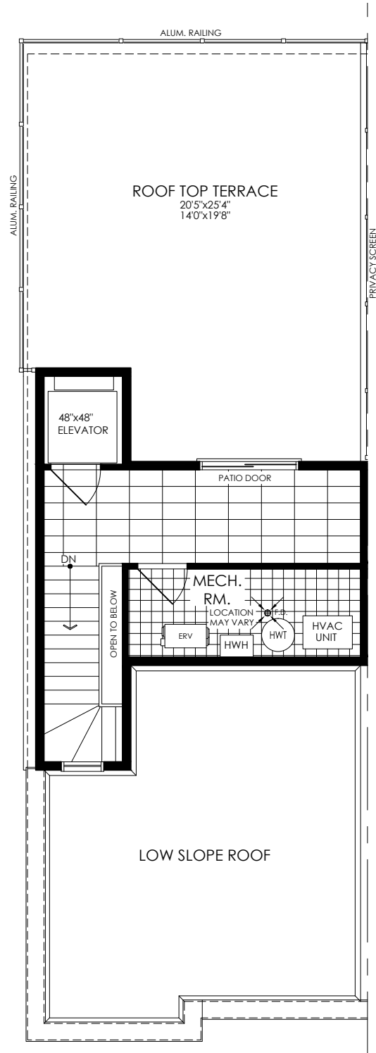
ROOFTOP/TERRACE • ELEV. B
