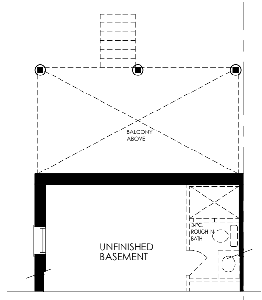
PARTIAL BASEMENT W/ WALK-OUT DECK COND. • ELEV. A
