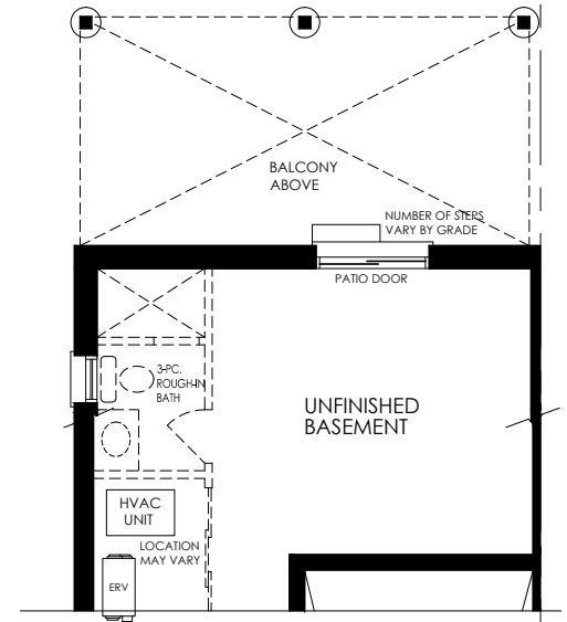
PARTIAL BASEMENT W/ WALK-OUT BASEMENT COND. • ELEV. C
