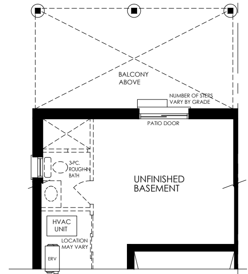
PARTIAL BASEMENT W/ WALK-OUT BASEMENT COND. • ELEV. B
