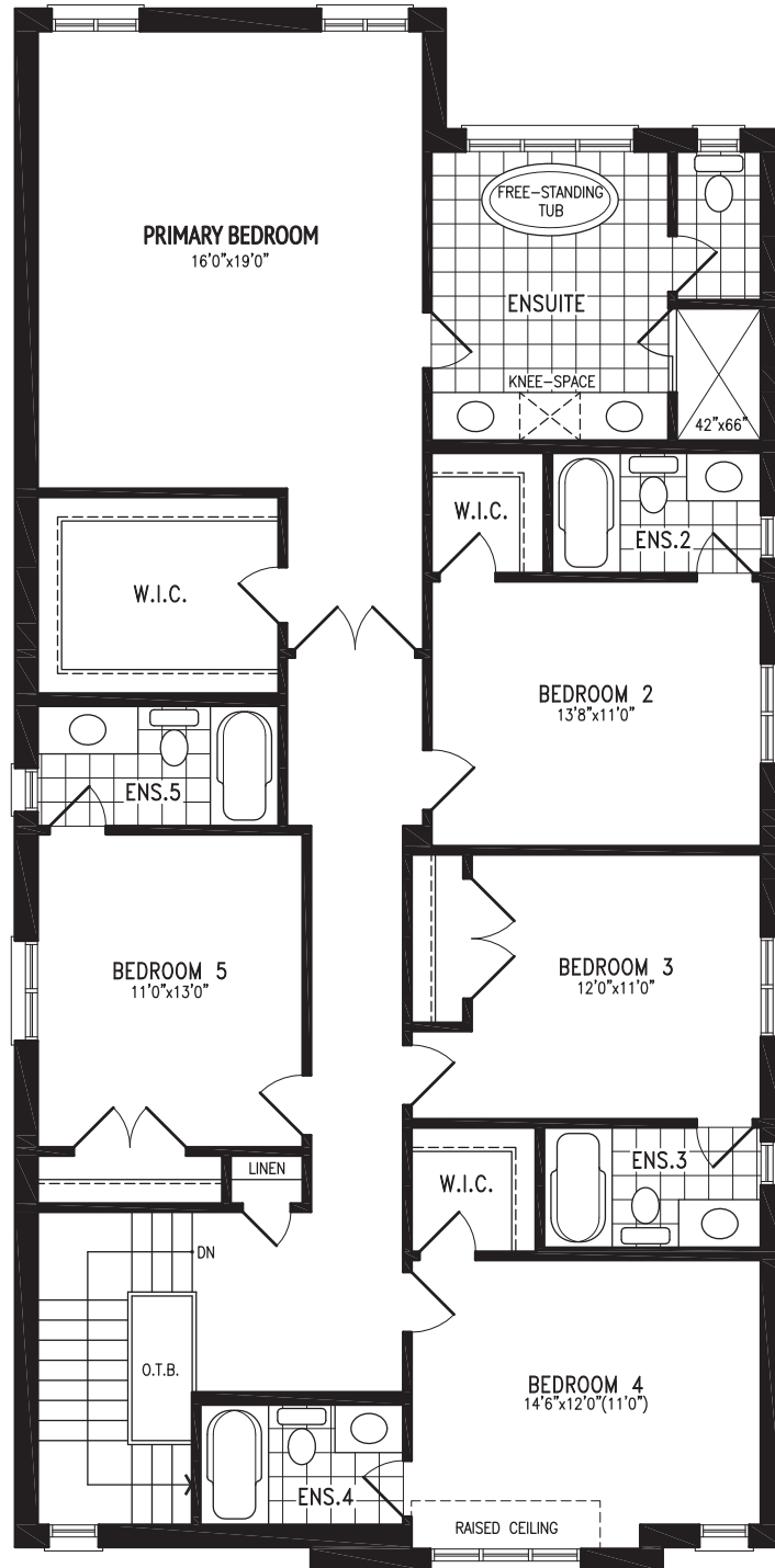
Elevation B SECOND FLOOR
