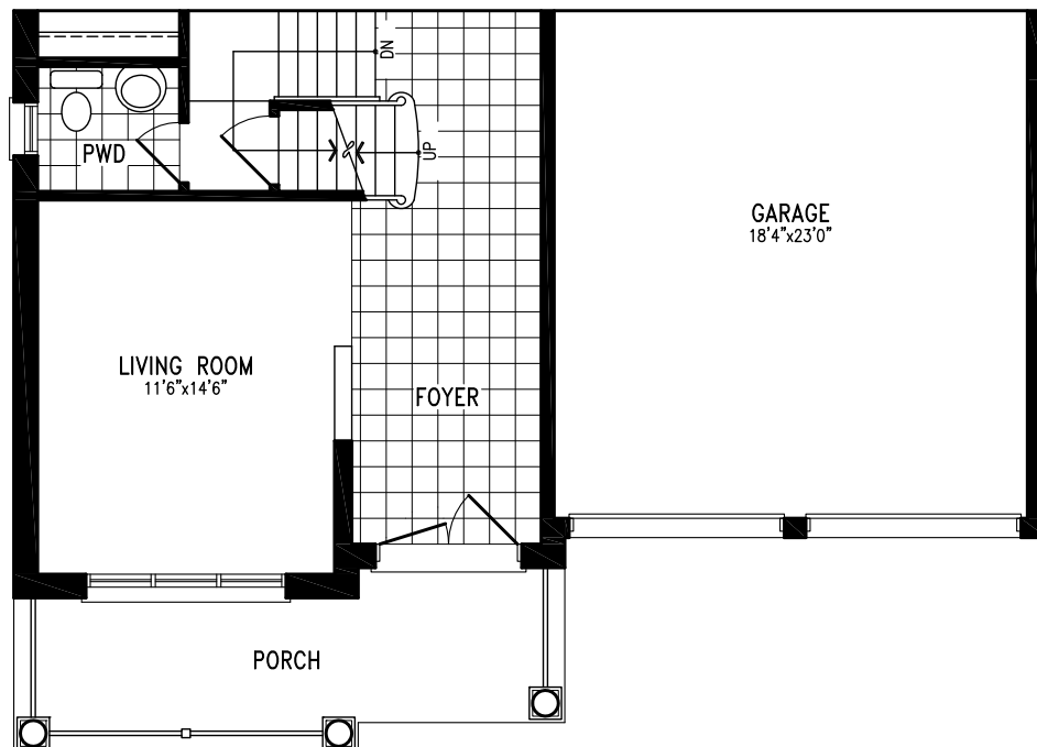
Elevation C PARTIAL GROUND FLOOR
