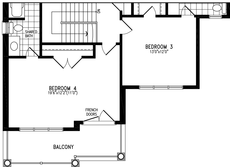
Elevation C PARTIAL SECOND FLOOR
