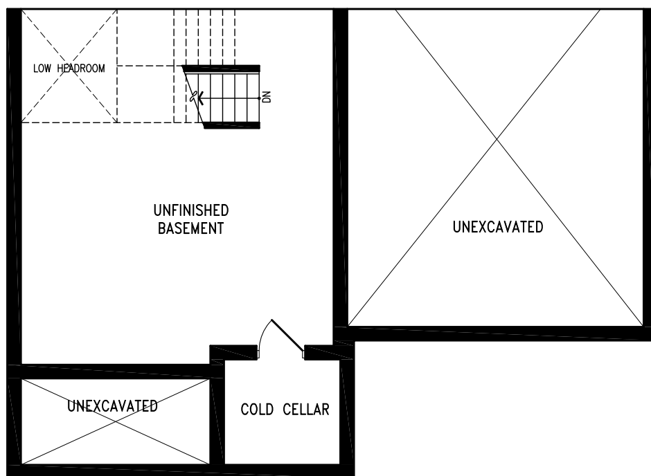
Elevation C PARTIAL BASEMENT
