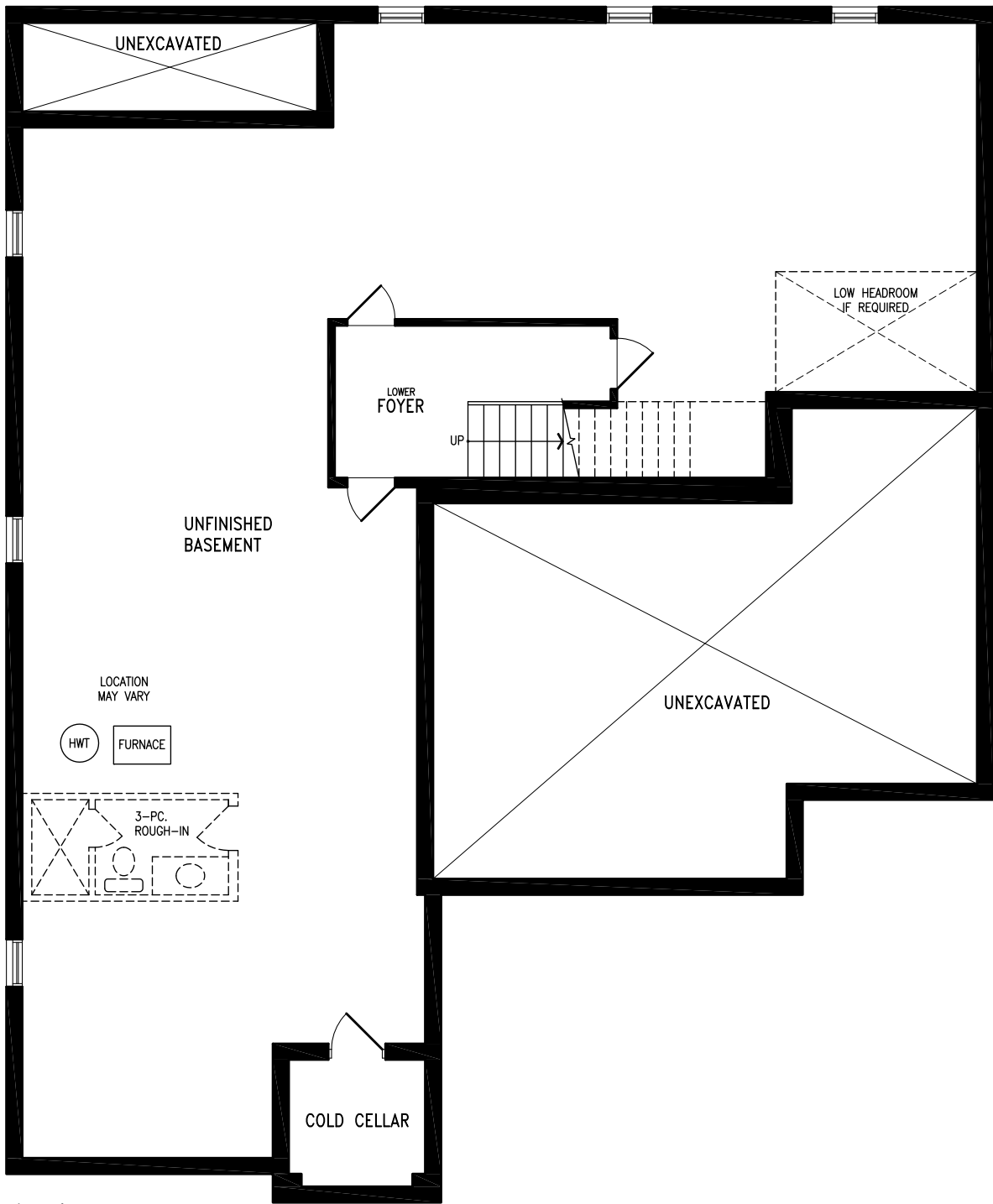
Elevation C BASEMENT
