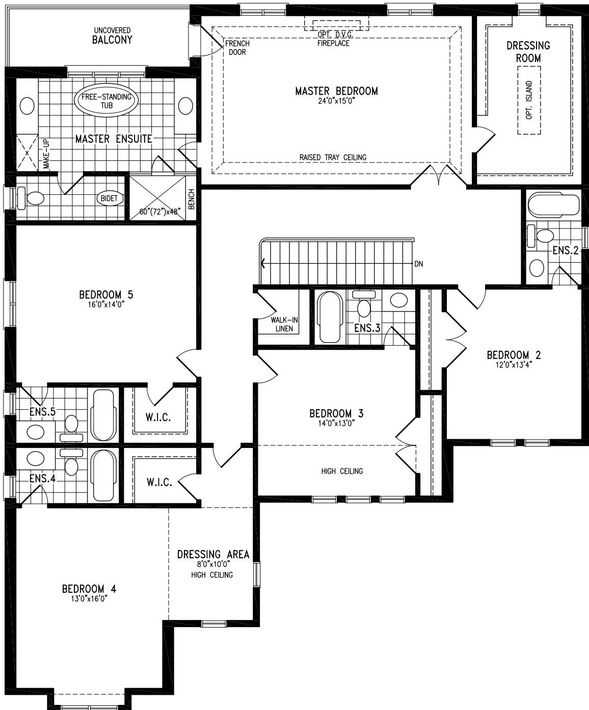
Elevation B OPTIONAL 5 BEDROOM SECOND FLOOR
