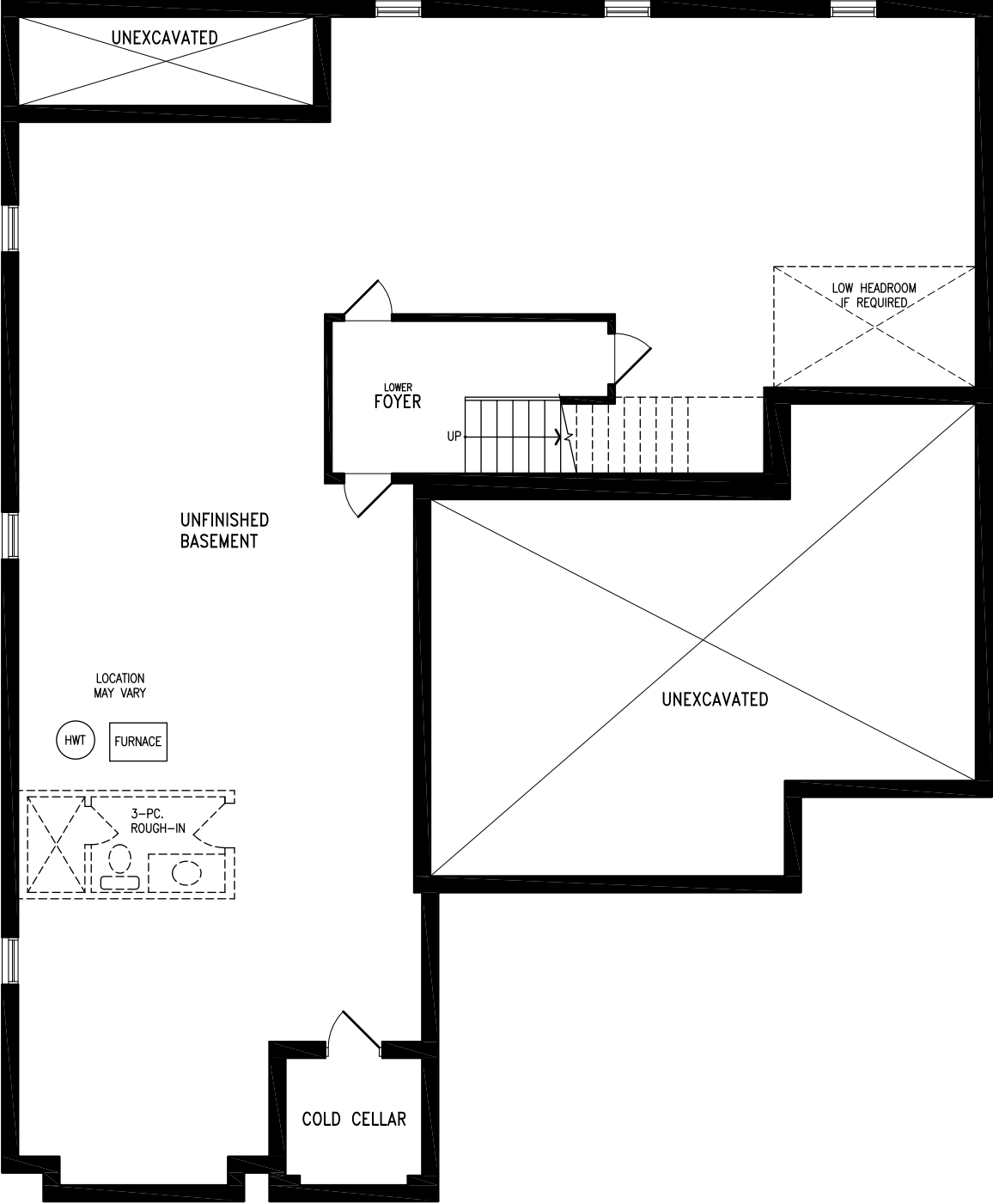
Elevation A BASEMENT
