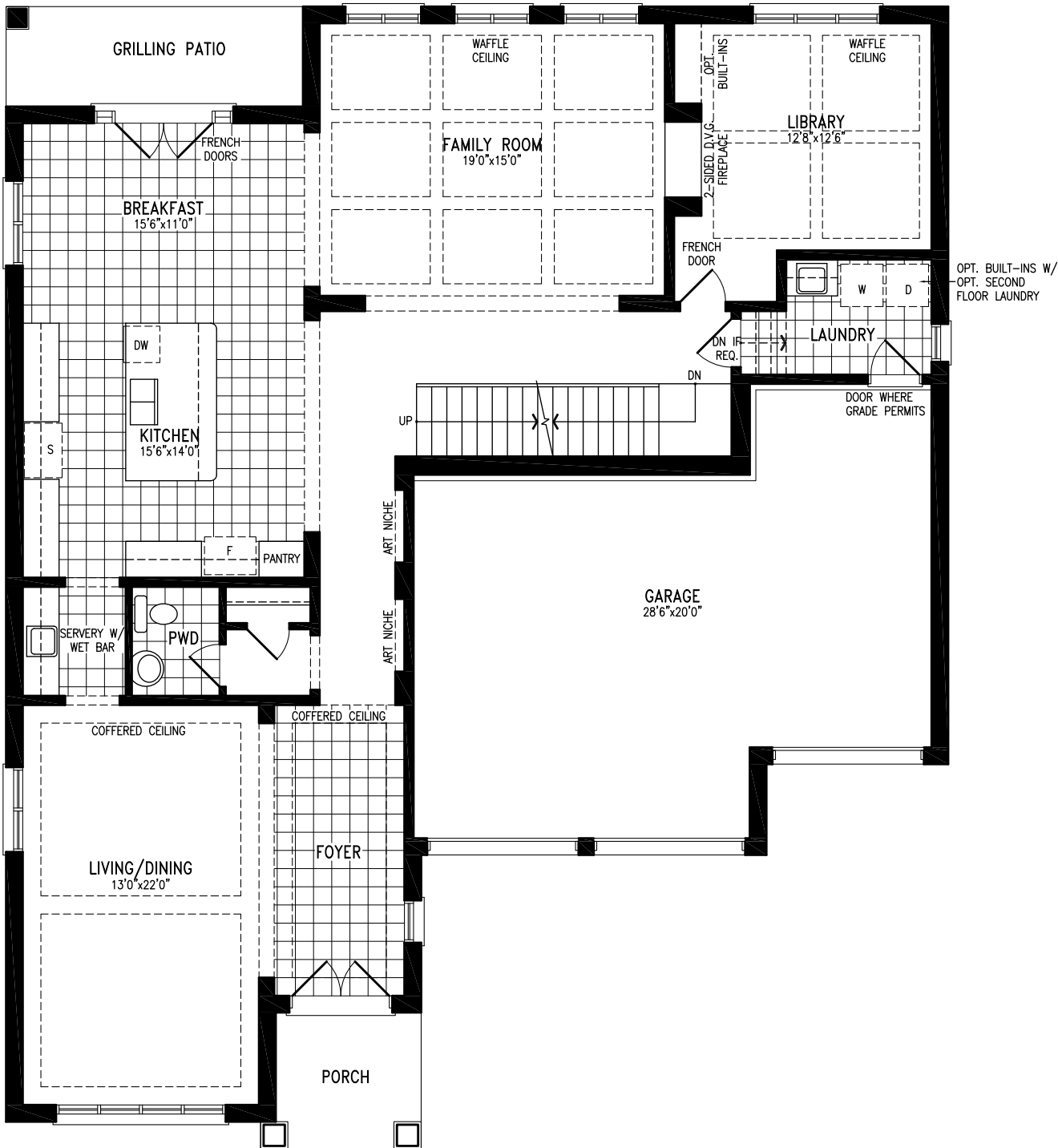
Elevation C GROUND FLOOR
