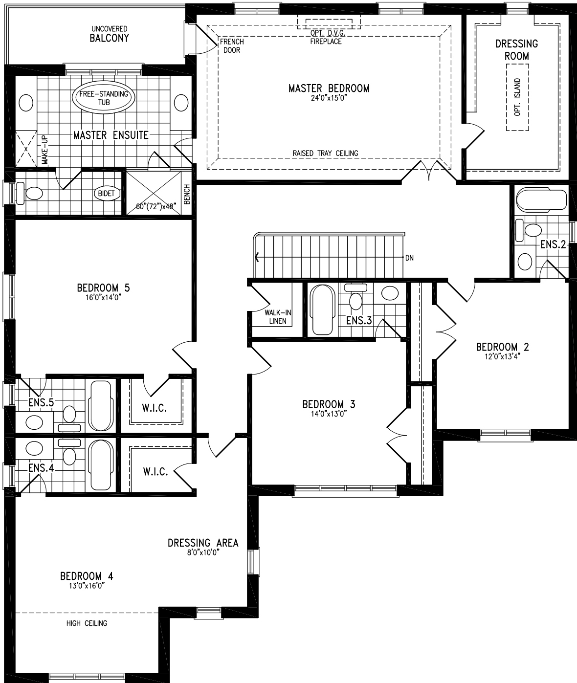
Elevation C OPTIONAL 5 BEDROOM SECOND FLOOR
