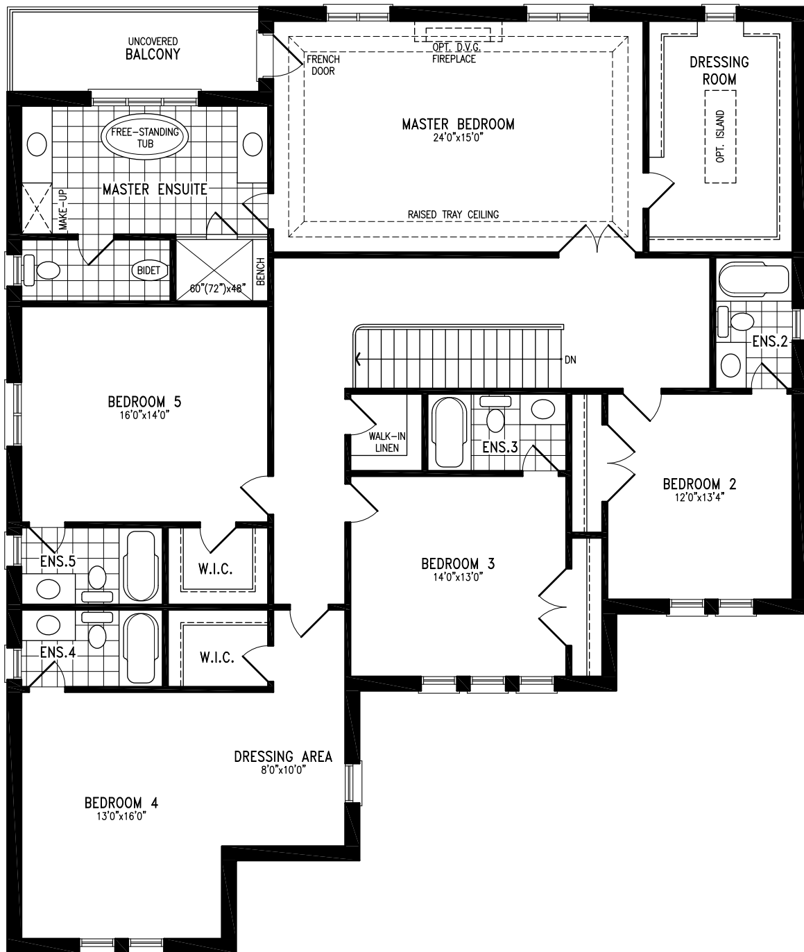
Elevation A OPTIONAL 5 BEDROOM SECOND FLOOR
