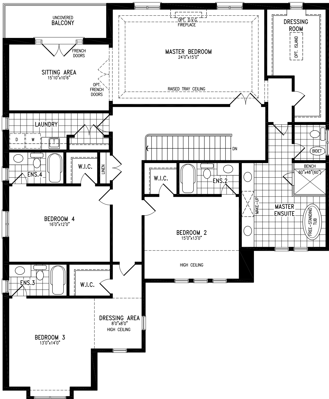
Elevation B OPTIONAL 4 BEDROOM W/LAUNDRY SECOND FLOOR
