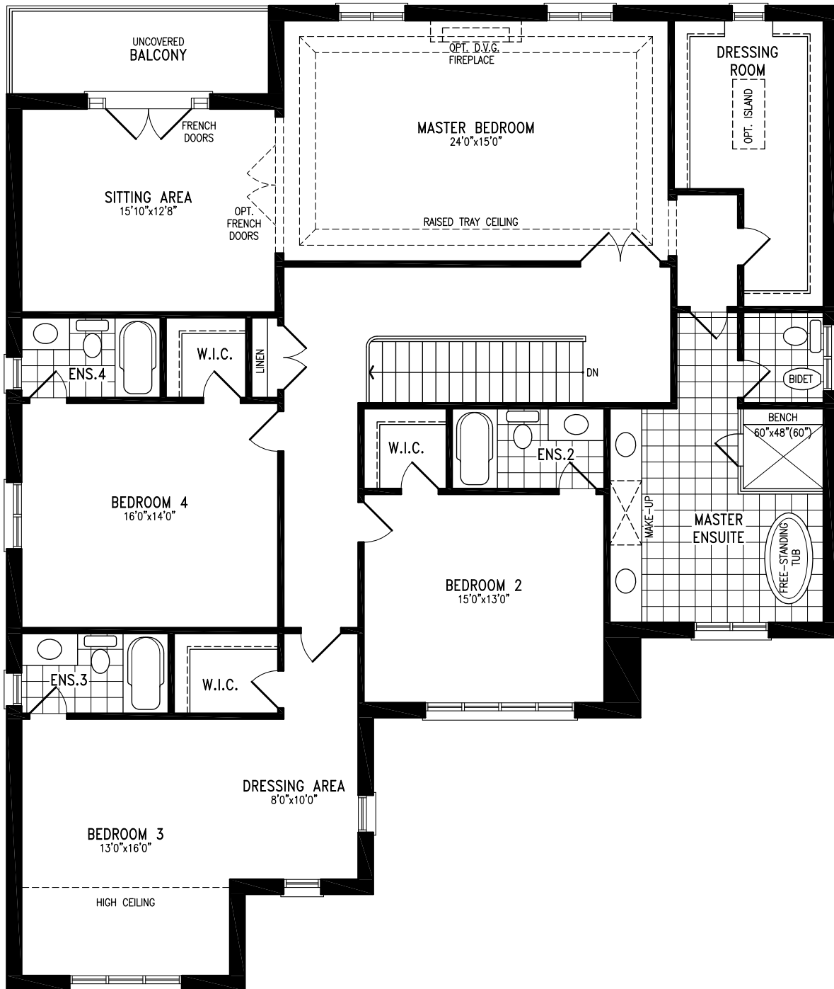
Elevation C STANDARD 4 BEDROOM SECOND FLOOR
