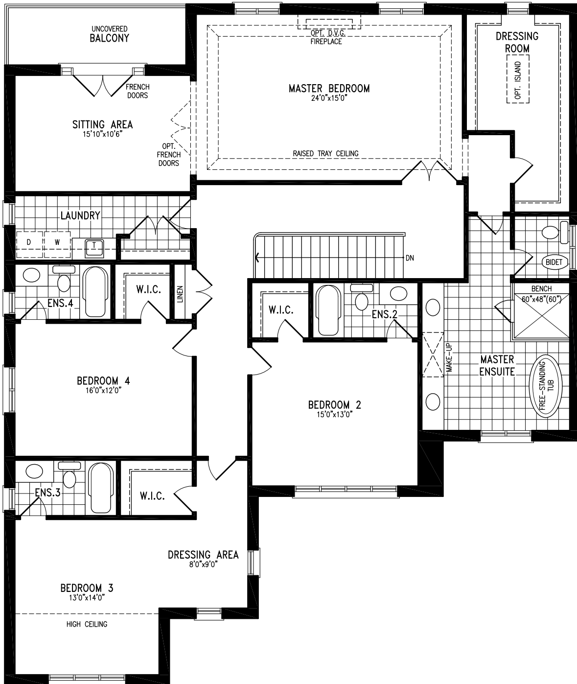
Elevation C OPTIONAL 4 BEDROOM W/LAUNDRY SECOND FLOOR
