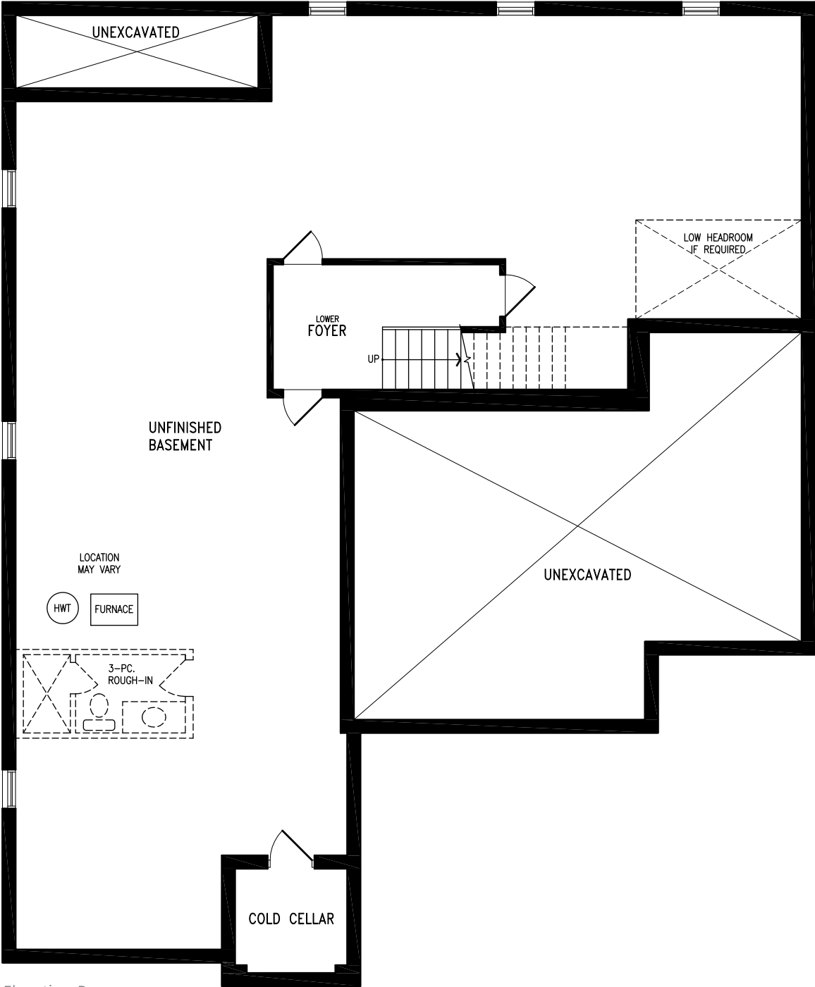
Elevation B BASEMENT
