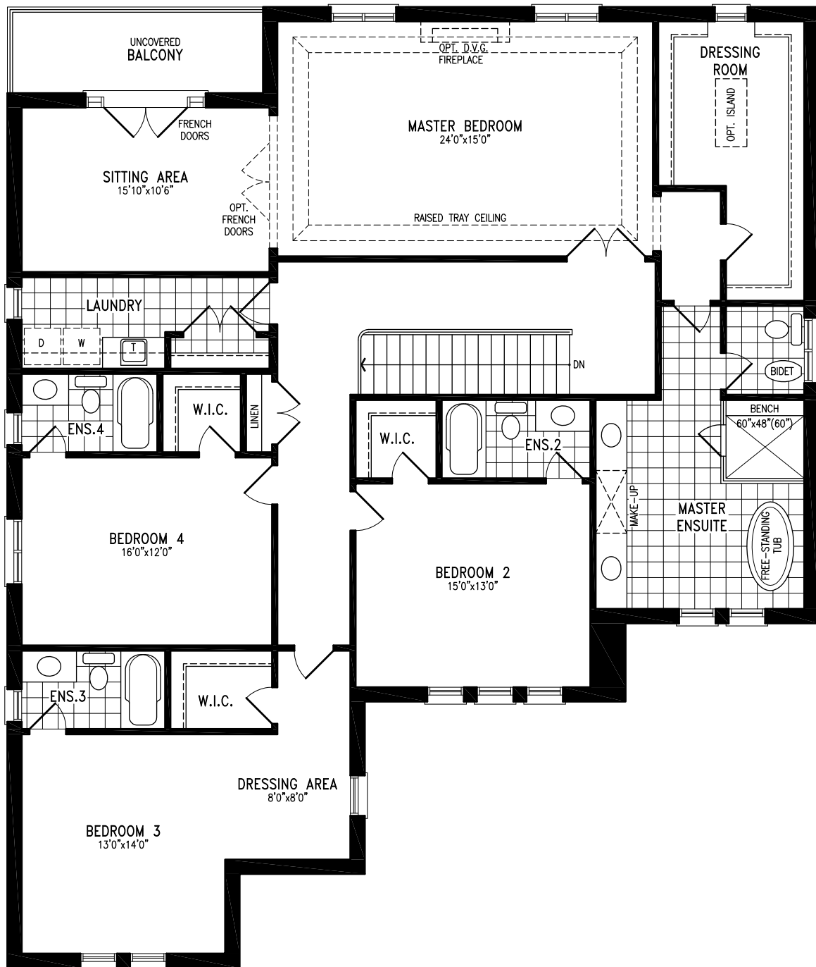
Elevation A OPTIONAL 4 BEDROOM W/LAUNDRY SECOND FLOOR
