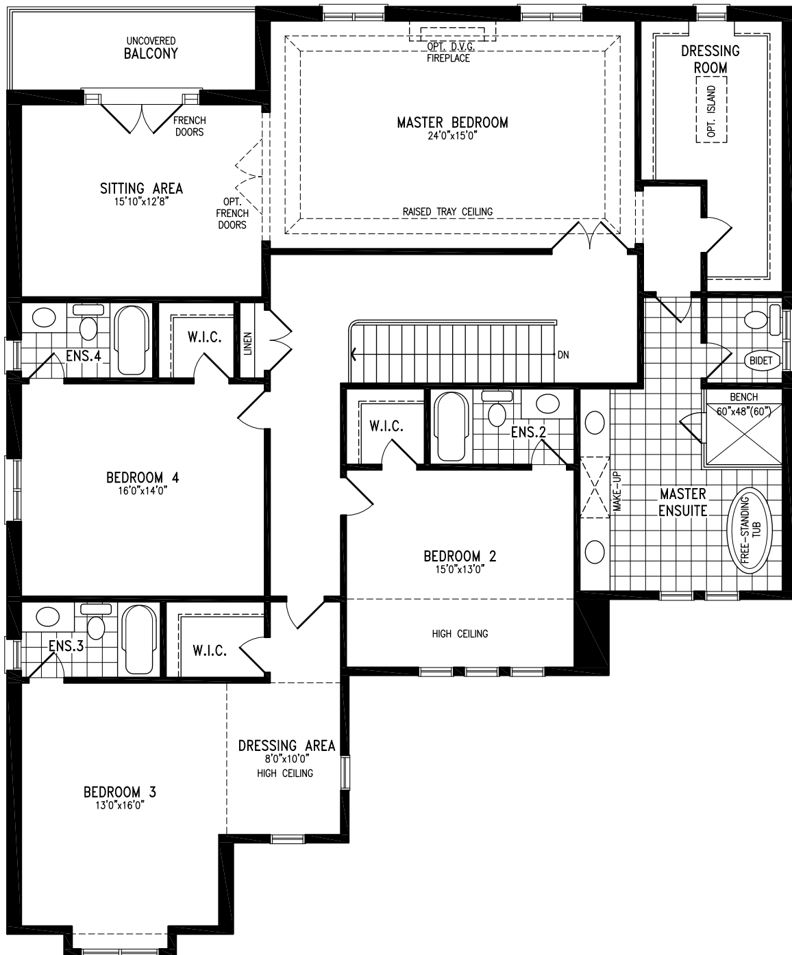
Elevation B STANDARD 4 BEDROOM SECOND FLOOR
