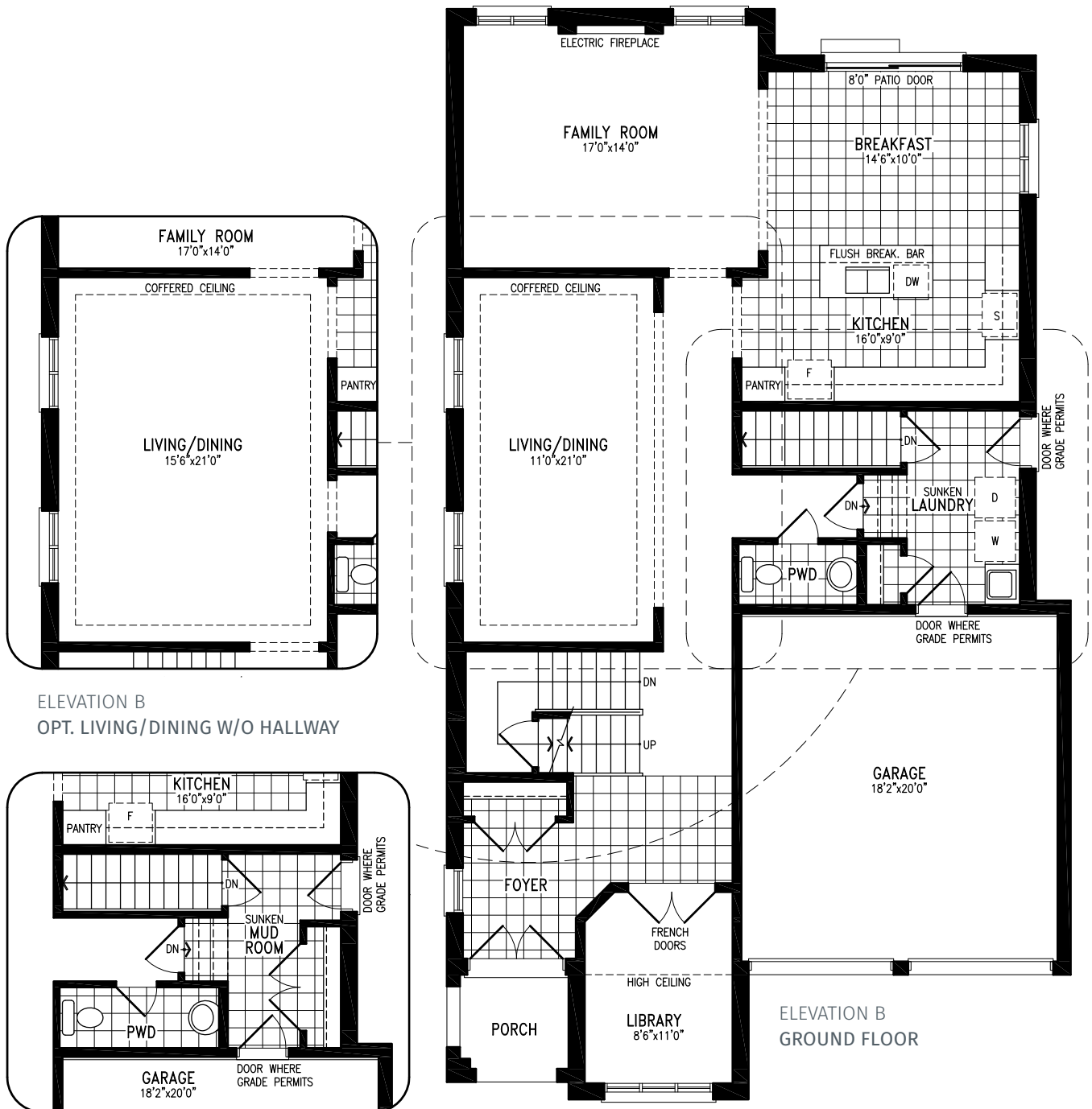
ELEVATION B OPT. MUD ROOM (Laundry to Basement or Second Floor)
