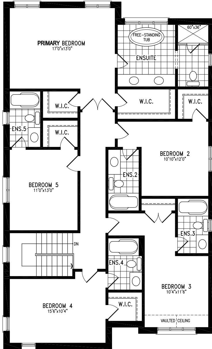
ELEVATION B OPT. 5 BEDROOM SECOND FLOOR
