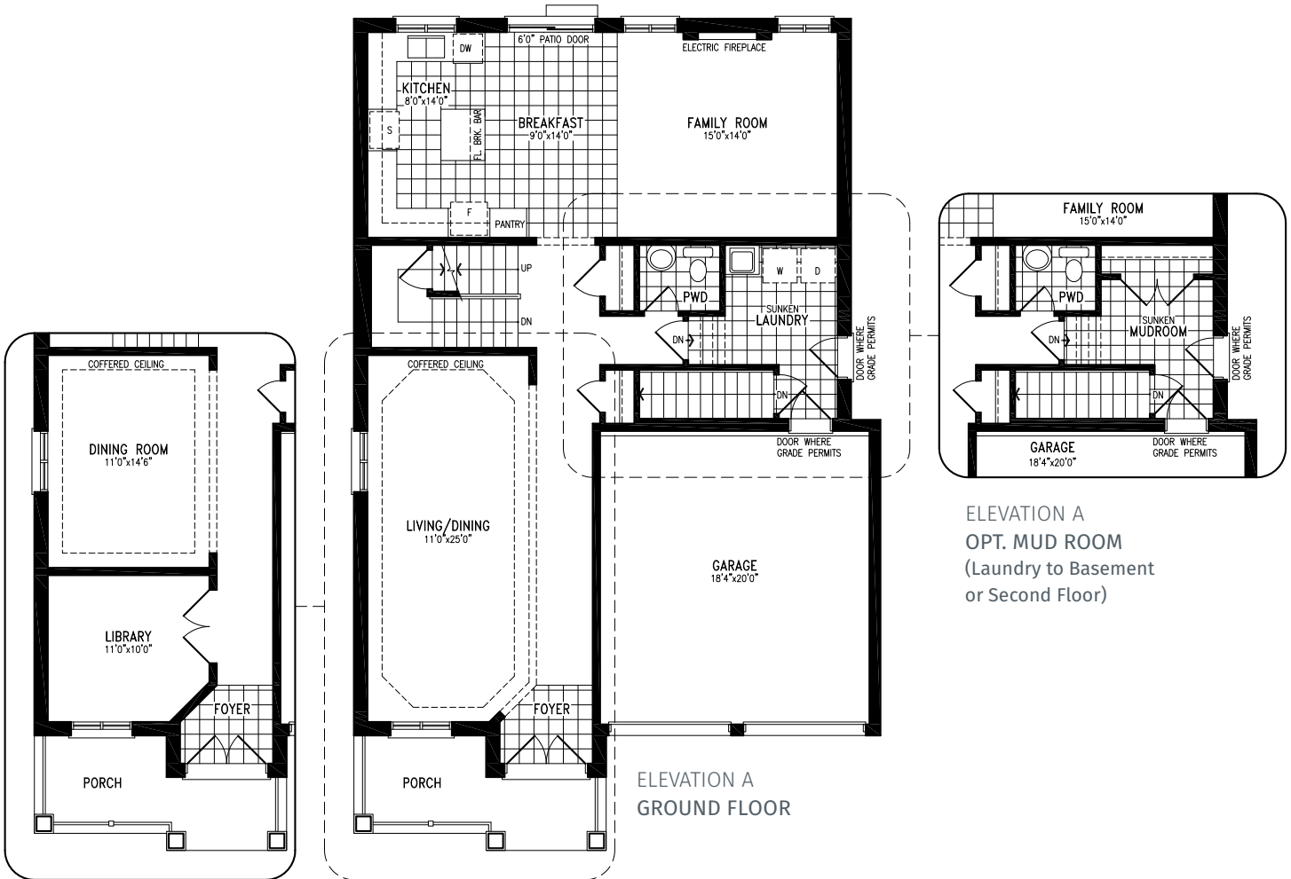
ELEVATION A OPT. DINING ROOM W/ LIBRARY
